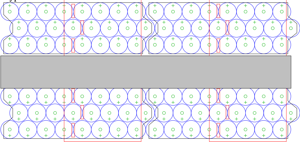
Type II PCB
