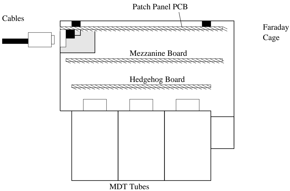
Cross-section through chamber from end
